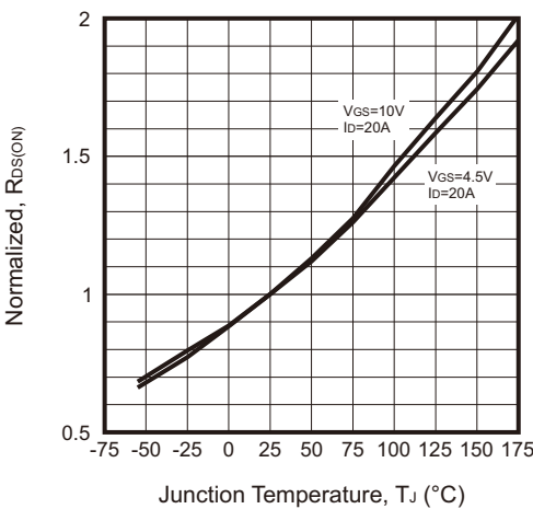
Fig.8 - Normalized R_{DS(ON)} vs T_J
