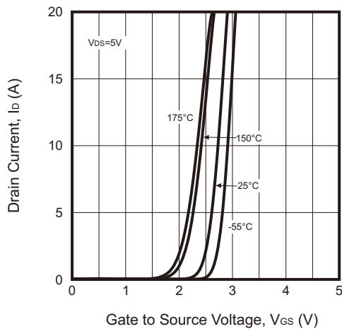
Fig.7 - Transfer Characteristics
